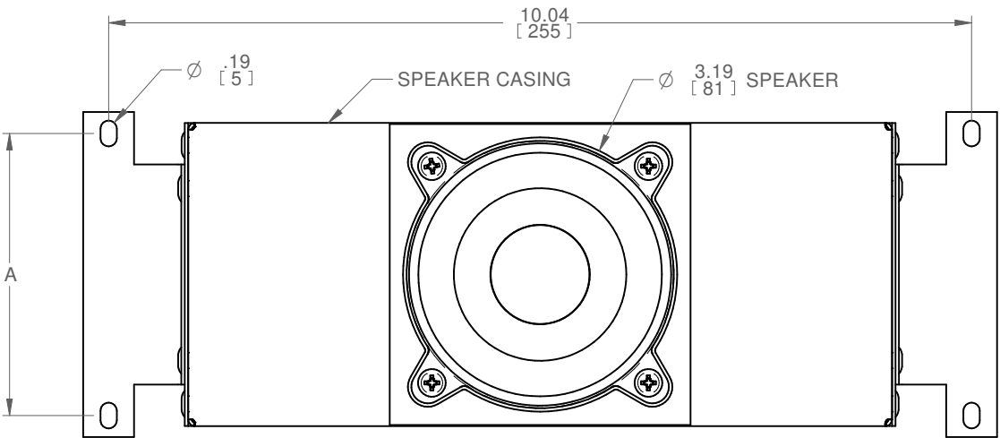
BOTTOM VIEW
