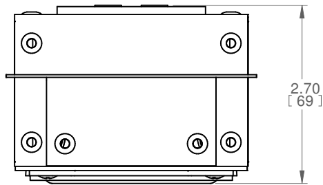
END VIEW
